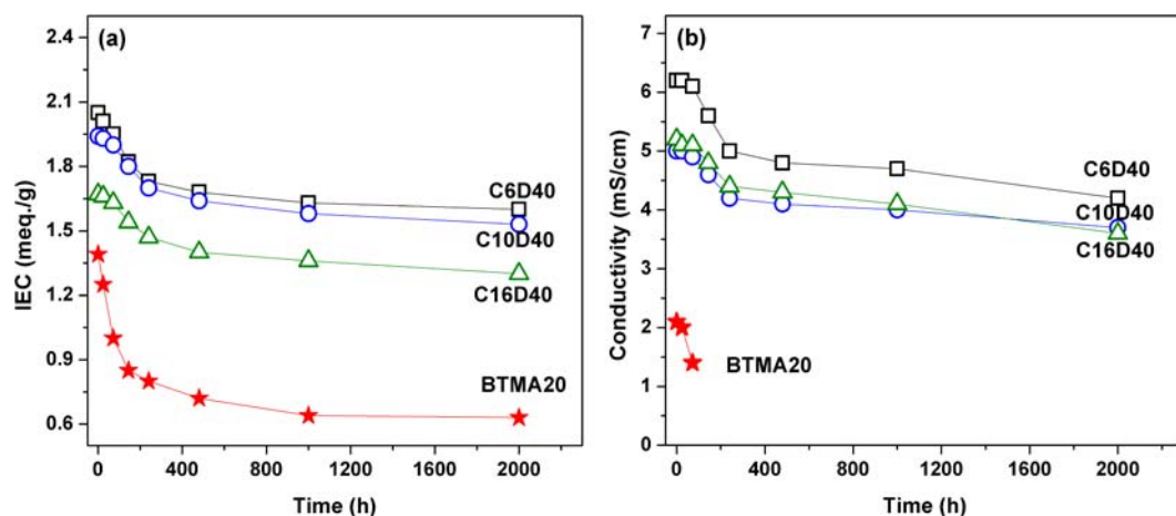
Figure 9. The changing trend in (a) IEC values and (b) bicarbonate of comb-shaped CyDx and BTMAx membranes after immersion in 1 M NaOH solution at 80 °C.
